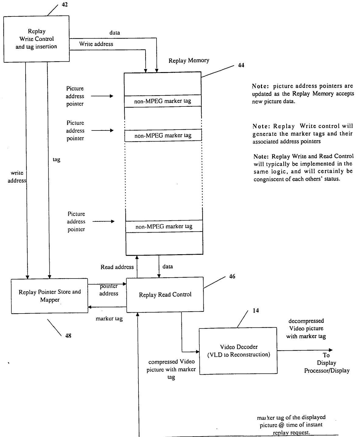
Figure 4: Major Components of the Instant Replay SubSystem
